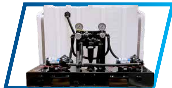
100 Gallon Low Profile Sprayer
